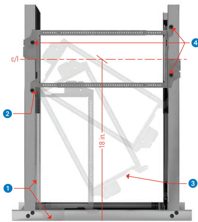
Telescoping bracket
