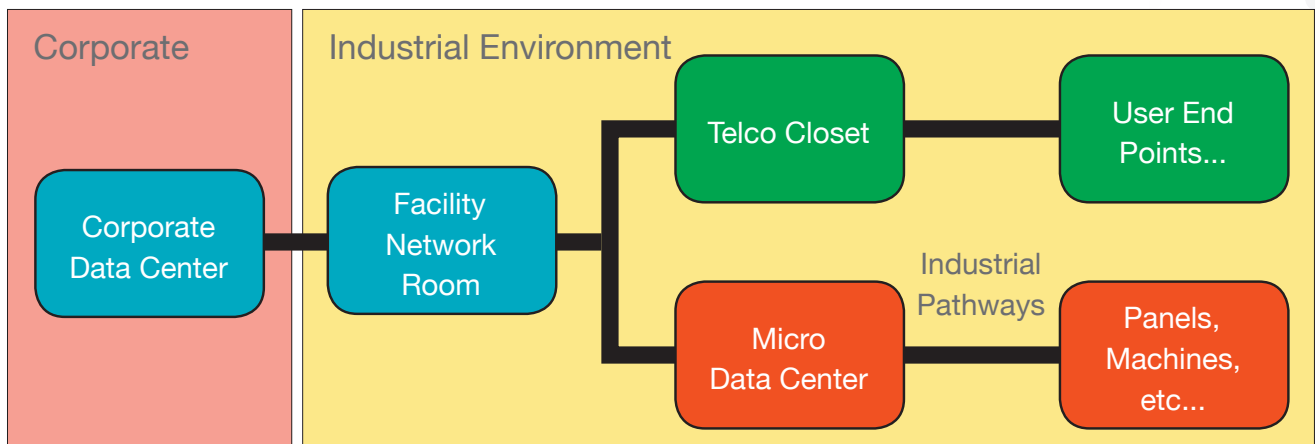
Figure 3. Block Diagram Indicating Location of Micro Data Center in Relation to the Data Center, Corp Network, Industrial Pathways, and Equipment Panels
