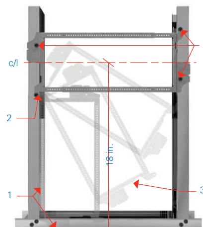
Telescoping bracket with BBA-4 and BBA added
